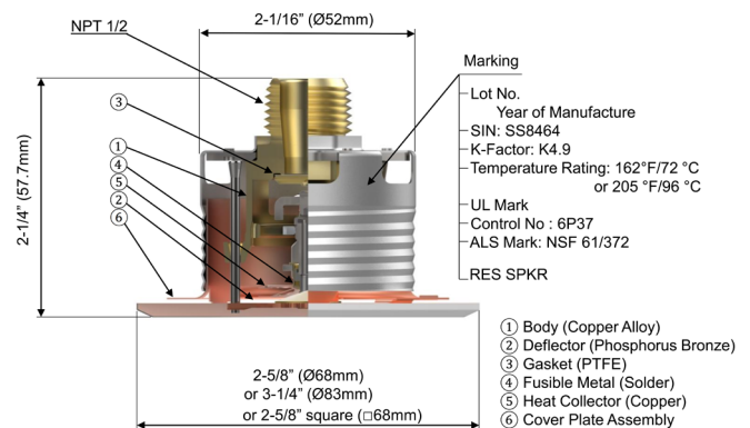
Figure 1: Model RC-RES K = 4.9
